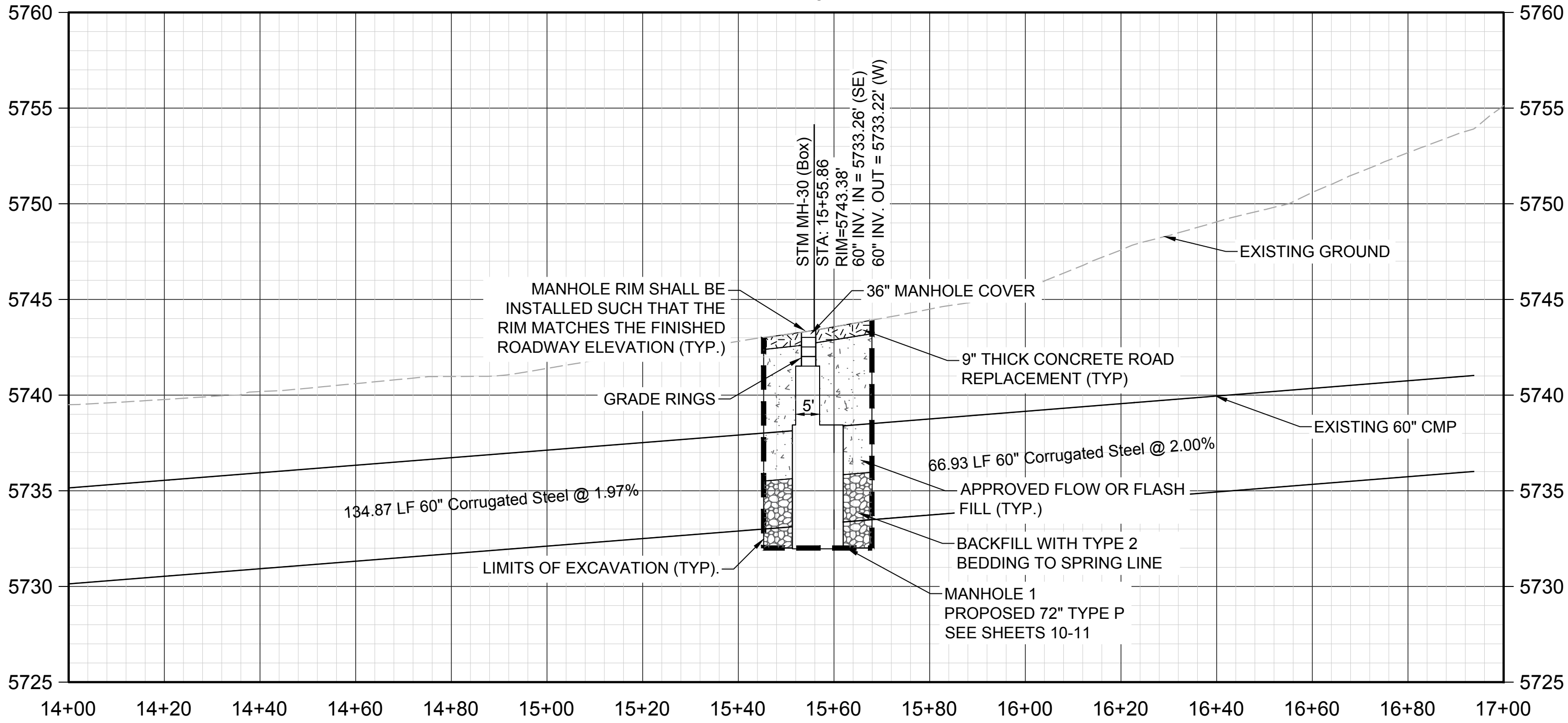
PROFILE OF EXISTING 60" CMP H: 1" = 20 V: 1" = 5
